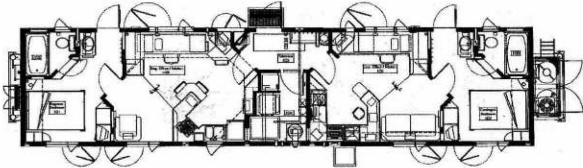
14'-0" x 60'-0" (skid) Wellsite
